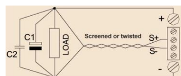
Figure 14.2: Remote Sensing (twisted sense lines)
