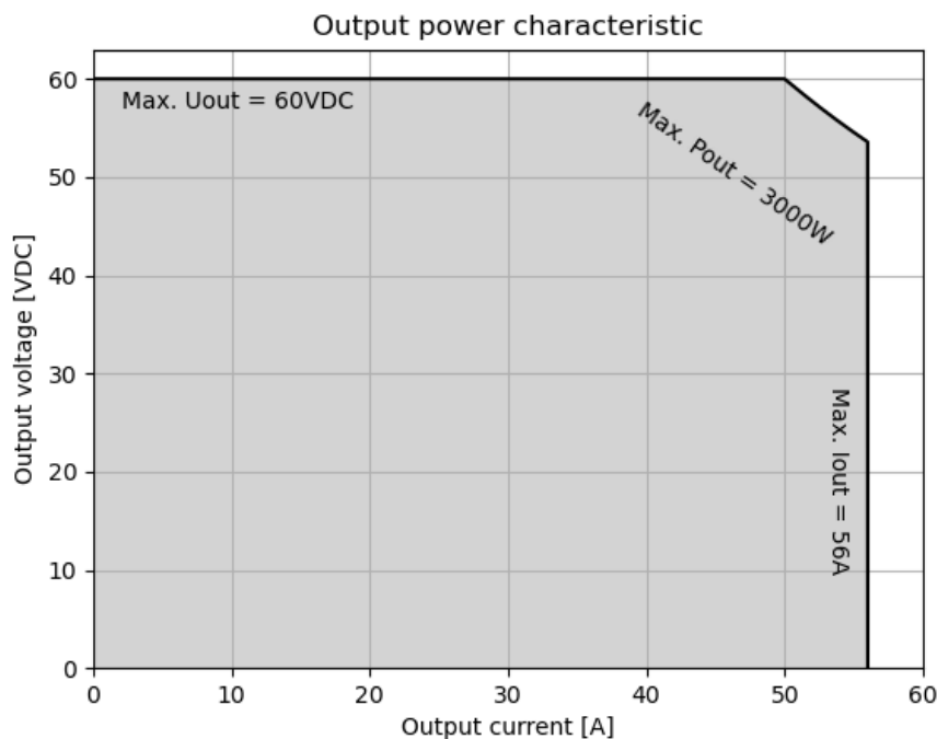
Figure 9.3: Output power DVCH3003-700-48
