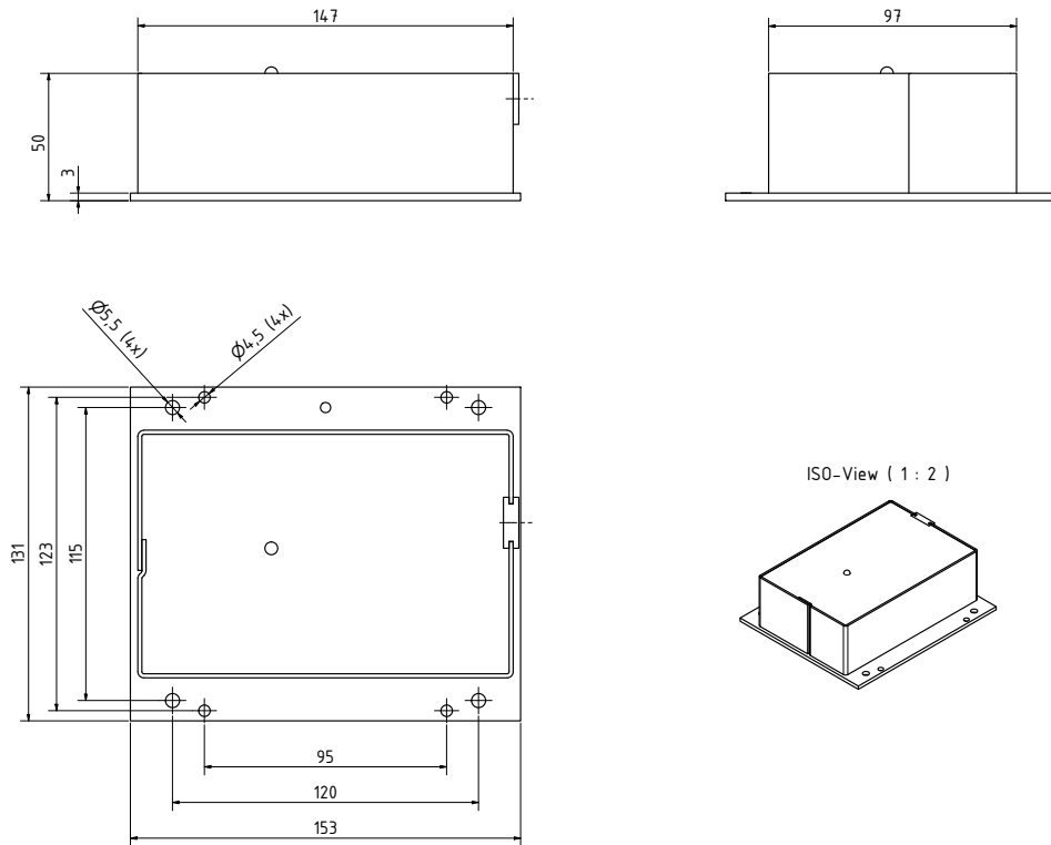
Figure 8.2: Dimensions derivate LED
