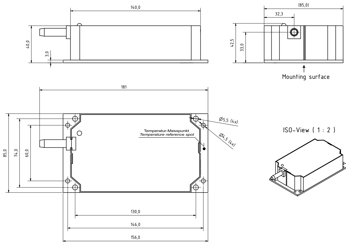
Figure 8.1: Dimensions
