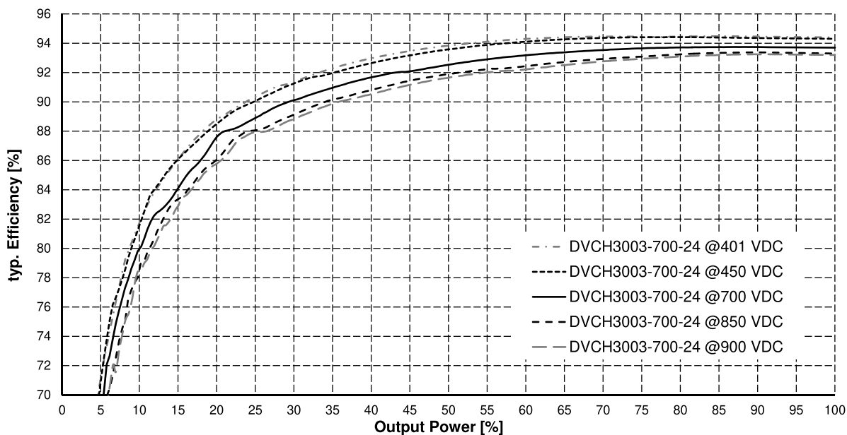
Figure 9.4: Efficiency as a function of output power
