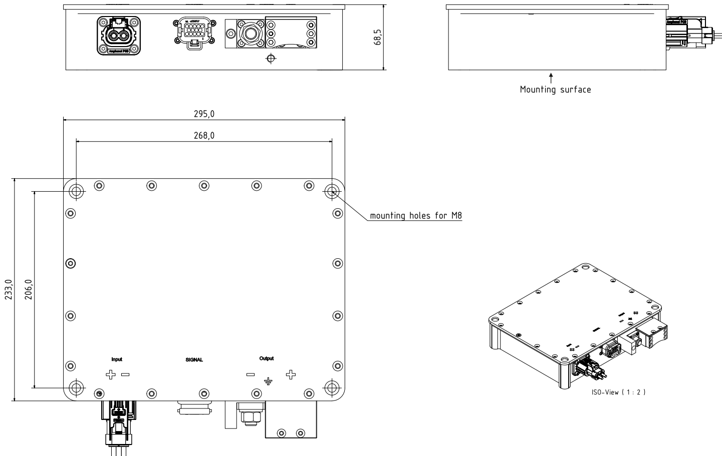
Figure 8.1: Dimensions
